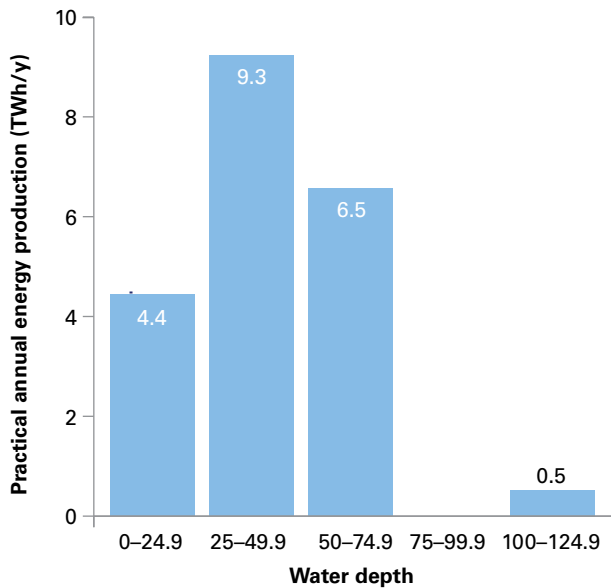
Figure 28 Distribution of average depths at UK tidal sites. The majority of the resource is in water depths 25m and over, though around 20% is still available at shallower depths. Only a small proportion of the resource is in depths over 75m
