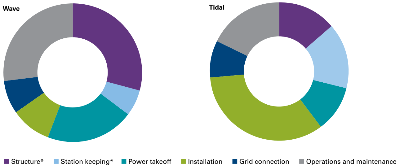
Figure 7a and 7b Indicative levelised cost of energy components for wave and tidal energy converters in an early commercial farm. The coloured segments are capital costs, while the grey segment represents O&M costs and includes all other spend including insurance and leases
