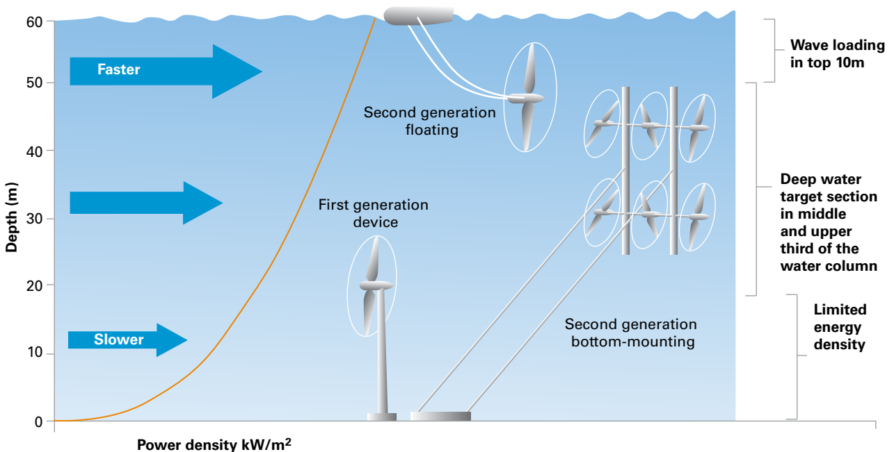
Figure 27 The high energy flows in a deep water column are nearer the surface, away from the bottom. A second generation of tidal turbines will be needed to access the optimum section of a deep water column – these might involve floating or neutrally buoyant devices
