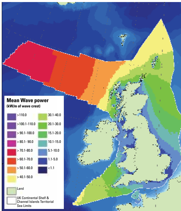
Figure 6 Average mean wave power (From the Atlas of Marine Renewable Energy Resources, published by BERR, 2008)
