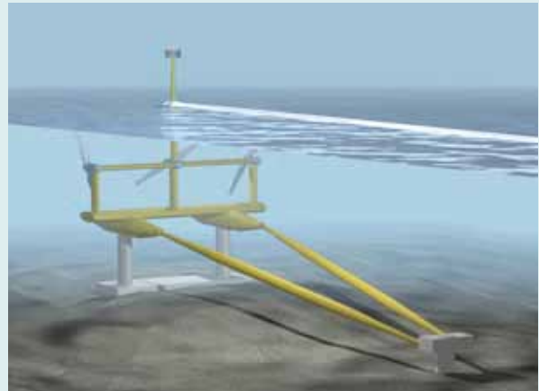
Figure 33: Second-generation tidal example: Marine Current Turbine's future device concept contains multiple rotors on a single support structure and single foundation.
