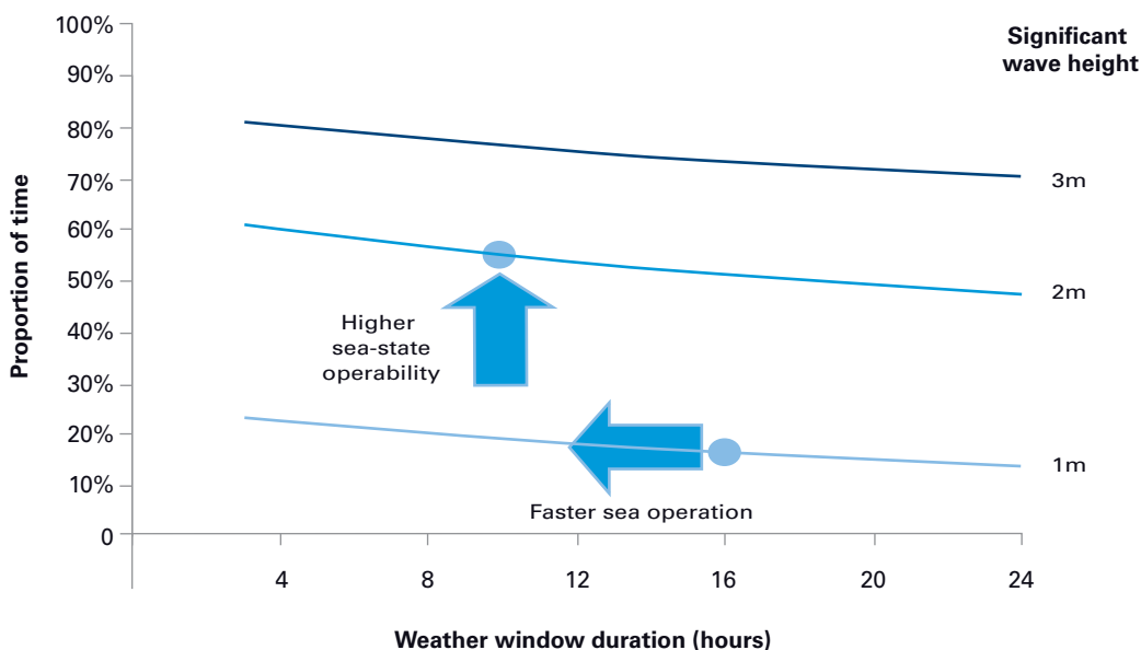
Figure 26 Sea operations are typically possible below a certain wave height – in the example shown lines are drawn indicatively for 1m, 2m and 3m for a site around Orkney. Device downtime can be reduced by increasing the range of sea states in which maintenance can be undertaken and by faster sea operations
