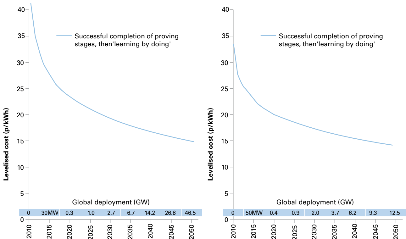
Figure 22a and 22b Baseline cost of energy reductions from wave and tidal devices, based on learning by doing only. Note that the roll-out rates for wave and tidal are different† 30
