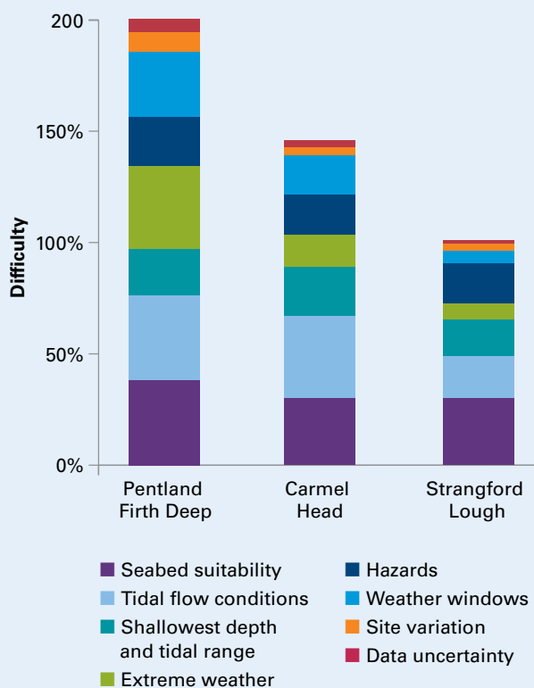
Figure 11 Example difficulty scores for three sites. All three sites have similarly difficult seabed conditions and marine hazards, but the Pentland Firth site is much more exposed leading to shorter weather windows and more extreme weather conditions. Notably, consistency and variability of the flow is problematic in the higher resource sites (Carmel Head and Pentland Firth)
