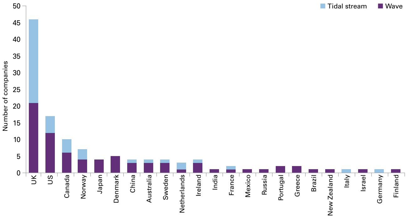
Figure 2 Indicative global wave and tidal activity
