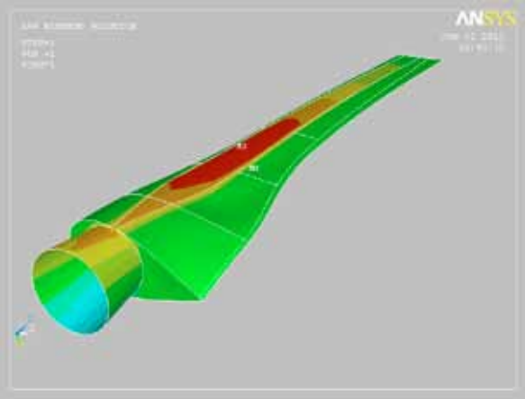
Figure 16 Carbon fibre tidal turbine blade project, by Aviation Enterprises Ltd. AEL makes blades for several tidal stream developers
