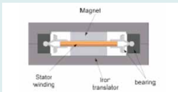
Figure 18 Linear generator for wave devices (Edinburgh University)
