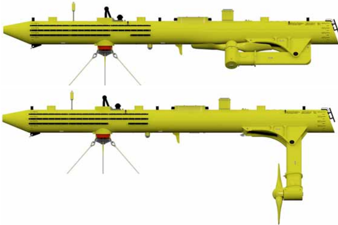
Figure 34 ScotRenewables' floating tidal device – shown in transportation/survival mode and generating mode – would be able to access high-energy resource near the surface of deep tidal streams, and should benefit from lower installation costs than fixed tidal turbines
