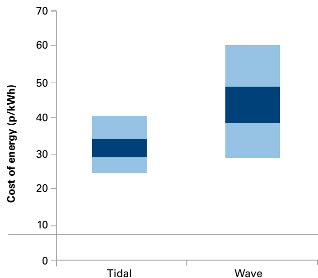
Figure 8 Baseline costs for benchmark first farm wave and tidal devices. These costs assume a discount rate of 15% and a lifetime of 20 years. The dark bars represent CoE at medium energy (upper bound) and high energy (lower bound) sites, using base case cost and performance assumptions; while the outer bars add optimistic and pessimistic cost and technical assumptions to these limits. Thus the lowest costs represent optimistic case cost and performance assumptions for devices sited in energetic locations
